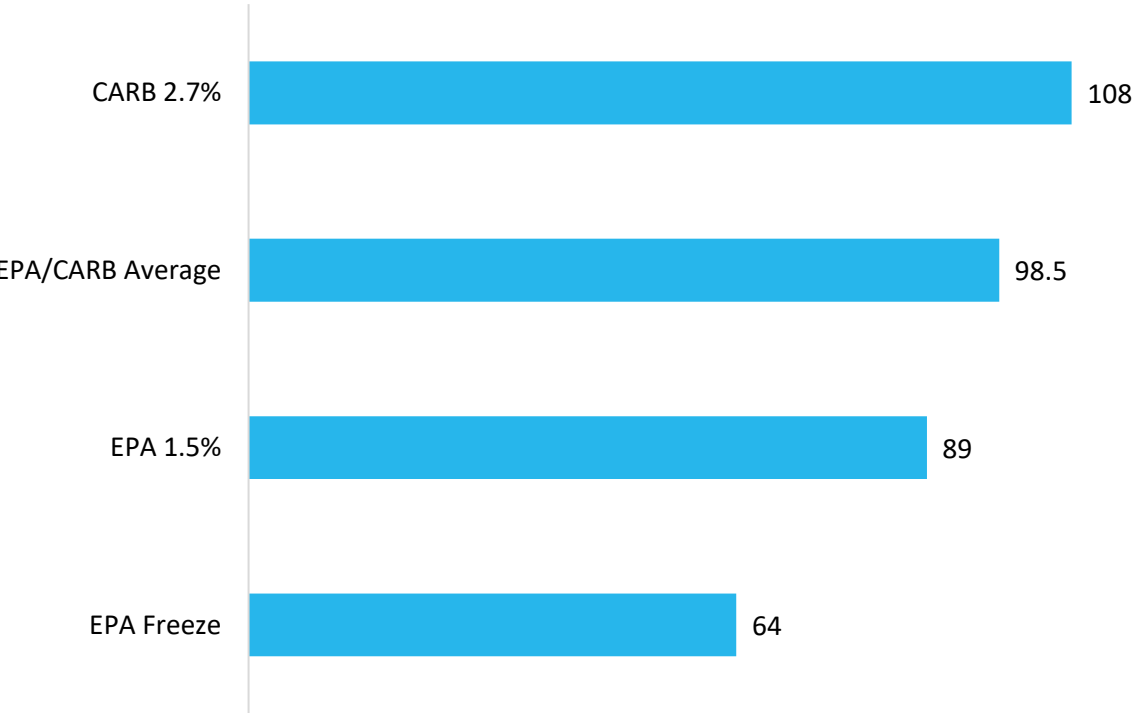
2018 -2026 CO2 Reduction Targets Real World Grams per Mile
